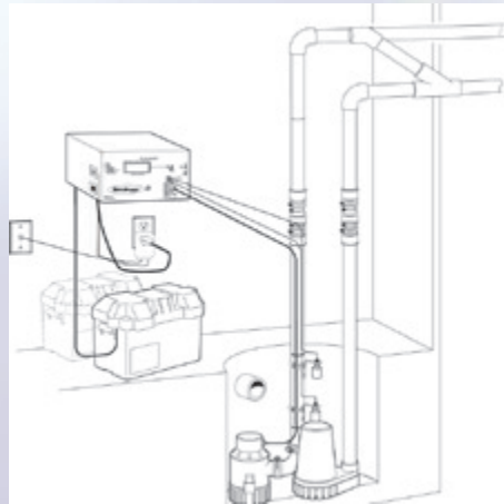
Single NexPump Installed as Backup System
