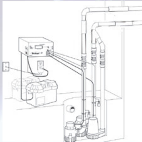
Dual NexPump Installed in Recommended Configuration
